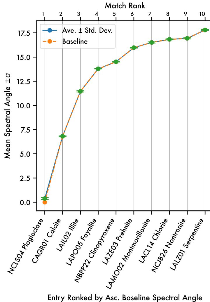
NCLS04 Plagioclase Mean Spectral Angle Match
